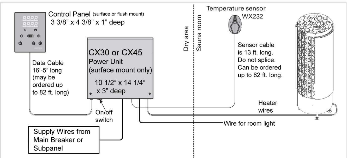
Figure 4. System components
