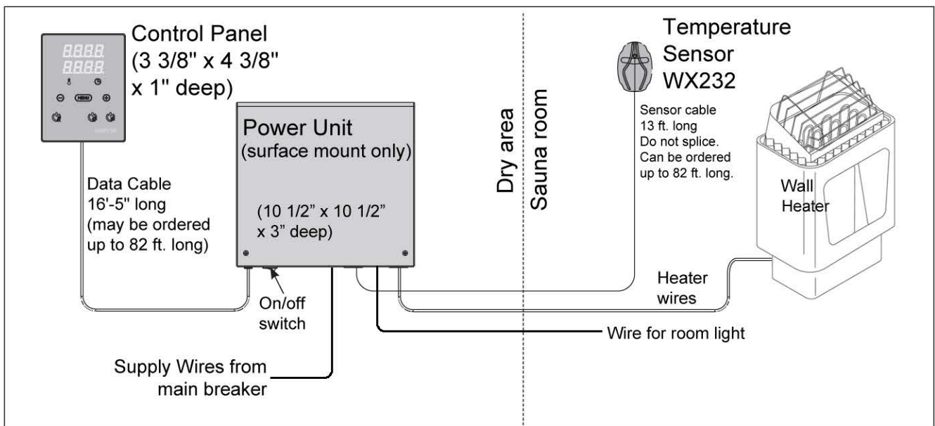
Figure 1. System components
